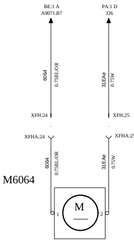
FAN, REHEATING SYSTEM
