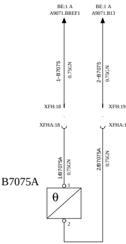
PASSENGER SENSOR, CLIMATE DOT
