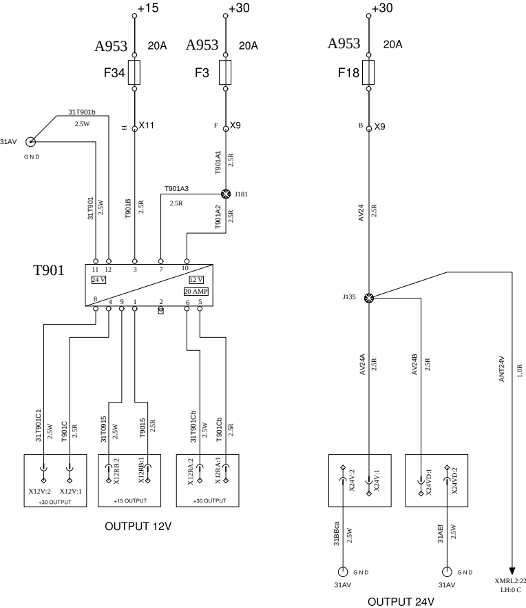
AUDIO AND VIDEO SUPPLY
