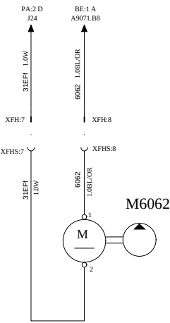
CIRCULATION PUMP, REHEATING SYS *This is included in Webasto*
